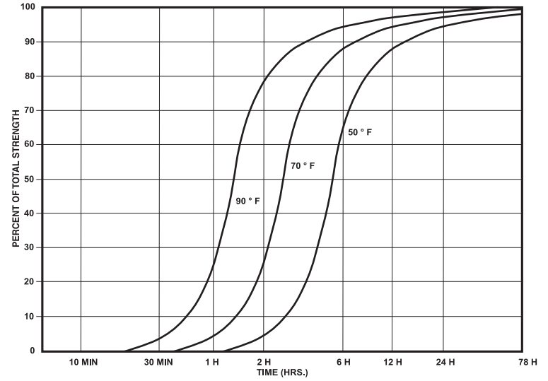
Graph V: Rate of cure at various temperatures
